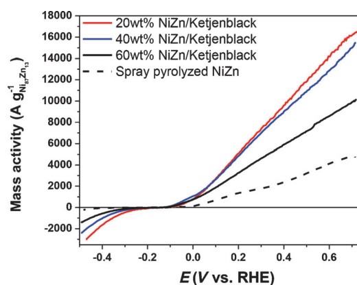
Figure 3. Cyclic voltammograms of NiZn catalysts with different metal loading compared to unsupported spray-pyrolyzed NiZn. Conditions: catalyst total loading 20 \mu\text{g} , 1 M KOH, 5 wt % hydrazine hydrate, 60 °C, \text{N}_2 purge, 1600 r.p.m.
